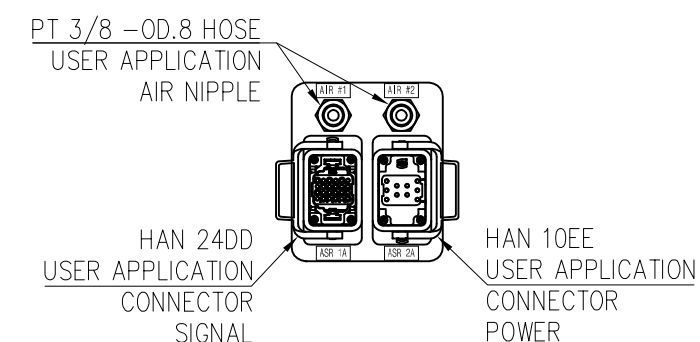
VIEW "D" (SCALE : 4/1)
