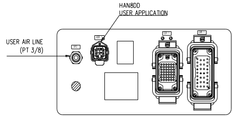
View D: Application cable connection part
